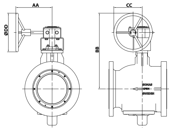
Ball segment valve type KVTF/KVXF with hand gear unit
